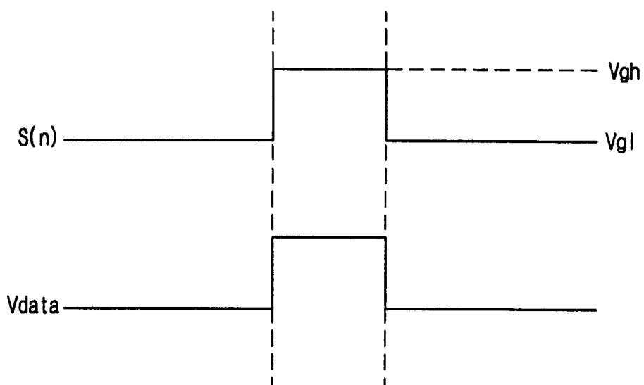
FIG. 2 RELATED ART
