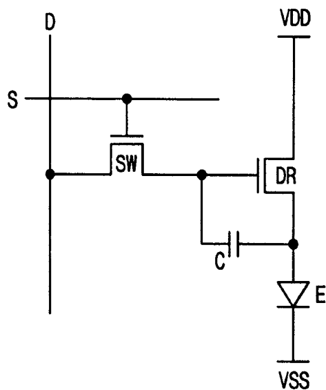
FIG. 2 RELATED ART
